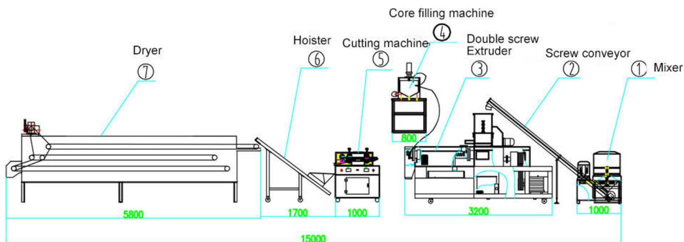
FLOW CHART OF 120KG-1200KG/H CORN PUFF MAKING MACHINE/ PRODUCTION LINE FOR RICE,
